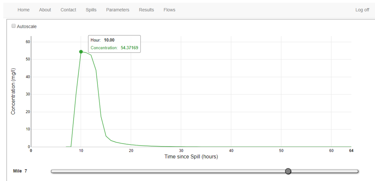
Figure 18 – Spill Plume at a particular distance (miles from spill location)
